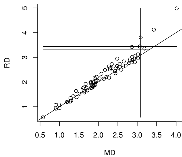
Figure 1: Prediction Regions for Buxton Data without Outliers
