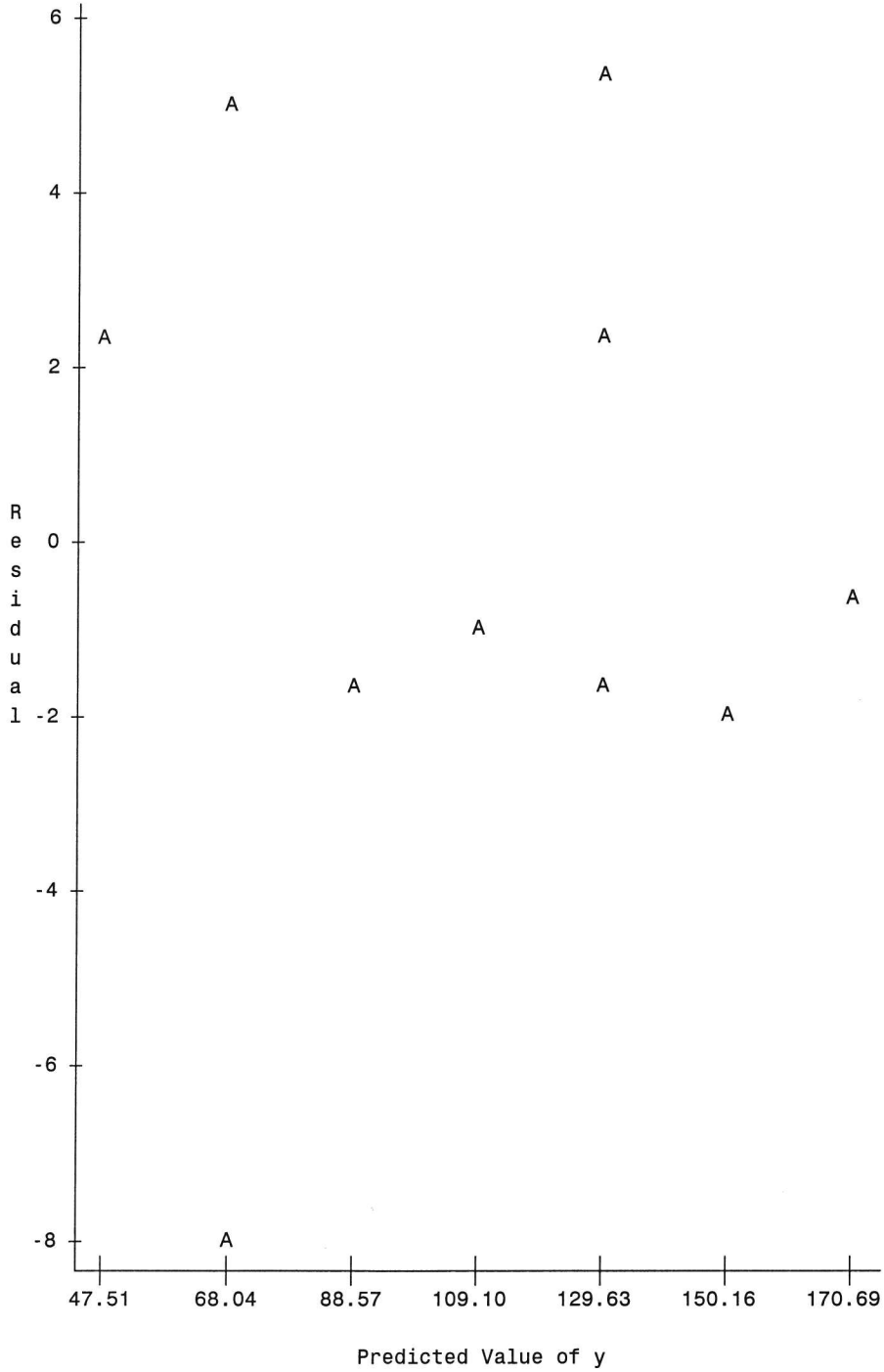
Plot of resid*pred. Legend: A = 1 obs, B = 2 obs, etc.
